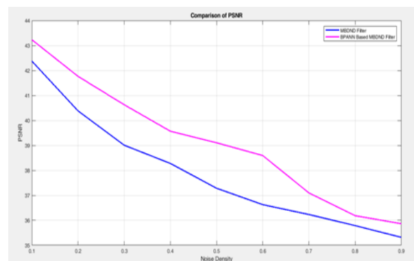
Fig 20: Comparison of PSNR
