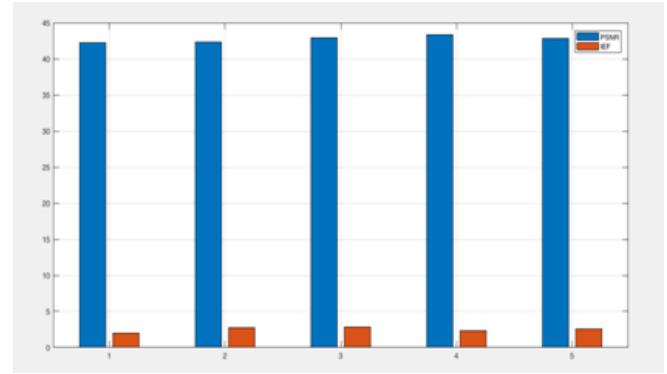
1=lena.jpg; 2=aktu.jpg; 3=aktu.png; 4=aktu.bmp; 5=aktu.gif Figure 7: Bar chart of PSNR & IEF
