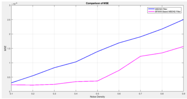
Fig 21: Comparison MSE
