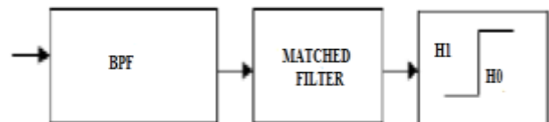
Fig.8: MFD Block Diagram
