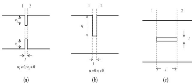
Figure 4: Top view: A pair of inductive discontinuities employed as planar filter coupling parts in rectangular waveguide. (a) Symmetric iris. (b) Asymmetric irises. (c) Centrally located bifurcation (axial strip) [1].
