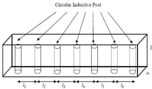
Figure 6: Geometry of a C_DWB filter with spacing l between irises, waveguide dimensions a and b [4].
