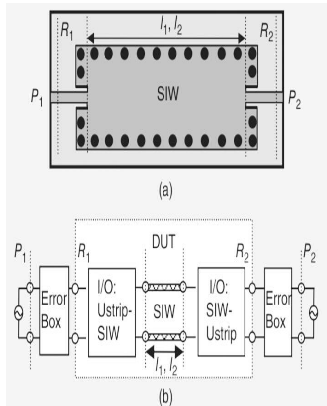
Figure 9: Block diagrams of numerical TRL calibration procedure for input/output structure (a) Input P1/output and (b) DUT [2].
