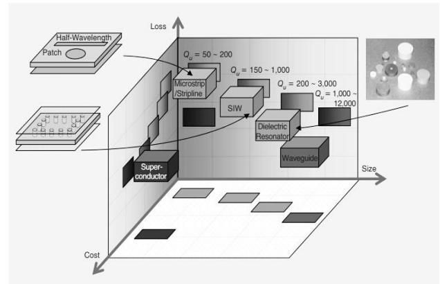
Figure 1: The relative insertion loss, size, and cost of various RF resonators [2].
