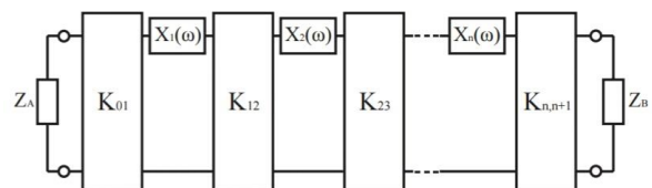
Figure 8: Band-pass ladder-type prototype circuit with identical resonators and impedance inverters [8].
