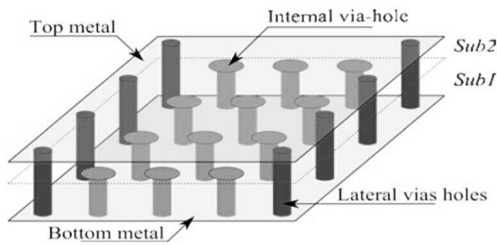
Figure 2: Topology of Slow-Wave SIW Technology [3].
