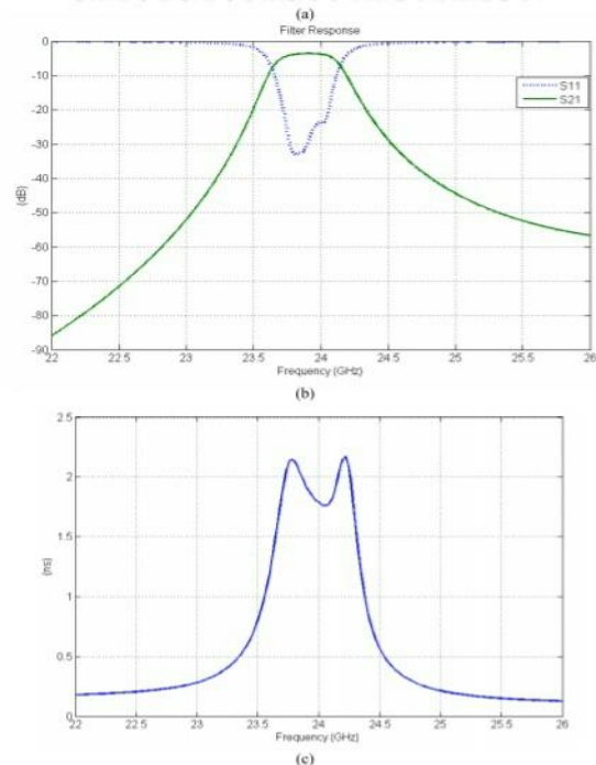
Figure 5: Metal insert filter. (a) HFSS model. (b) Filter response in HFSS. (c) Time delay [1].
