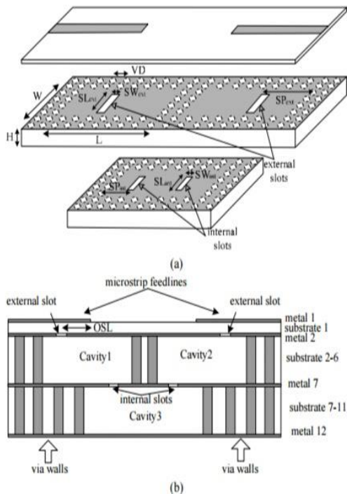
Figure 7: LTCC 3-pole cavity band pass filter employing slot excitation with an open stub: (a) 3-D overview, (b) side view of the proposed filter [9].
