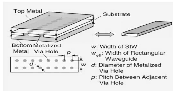
Figure 3: An SIW and its equivalent rectangular waveguide [2].
