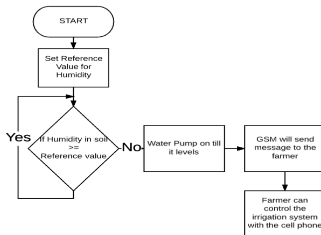
Fig.3. Flow Chart
