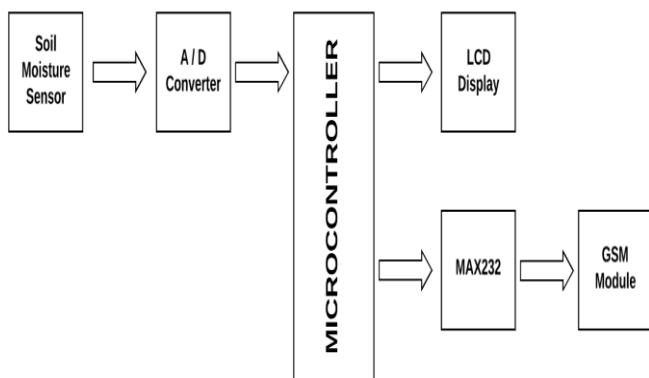
Fig.2. Block Diagram
