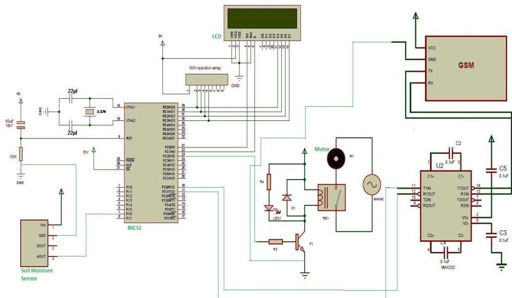
Fig.4. Circuit Diagram
