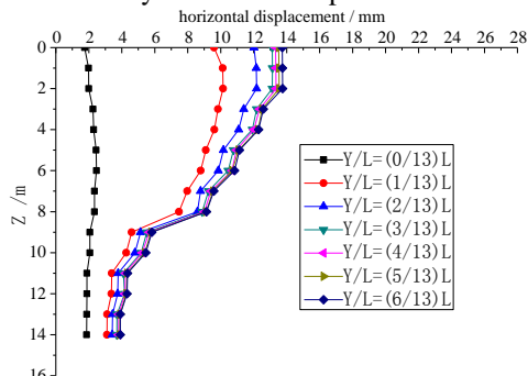
Figure 4.9 Horizontal displacement diagram of slope wall when C=1.5H
