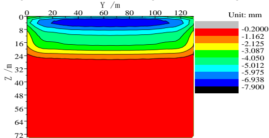
Figure 4.14 Nephogram of surface settlement diagram without building
