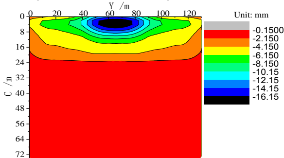
Figure 4.16 Nephogram of surface settlement diagram When C=0.5H
