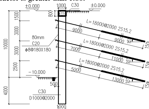
Fig. 2.2 Sectional diagram of pile anchor support system
