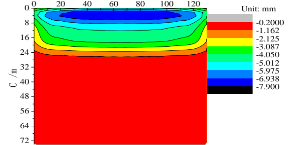
Figure 4.20 Nephogram of surface settlement diagram When C=1.5H
