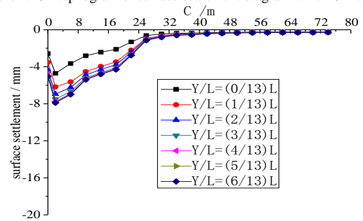
Figure 4.19 Surface settlement diagram when C=1.5 H
