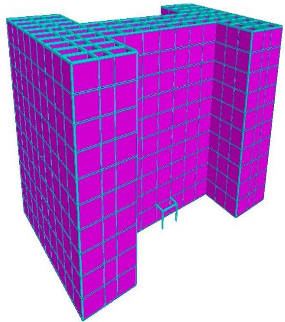
Fig .3 Frame with brick infill wall
