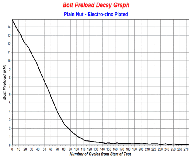
Figure no.2: Bolt preload decay graph
