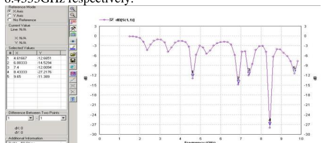
Fig. 11. Return Loss for Third Order
