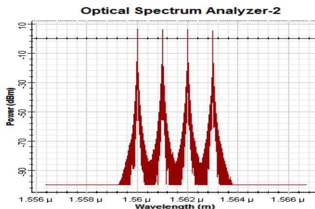
Figure 2: Multiplexed signal at OLT
