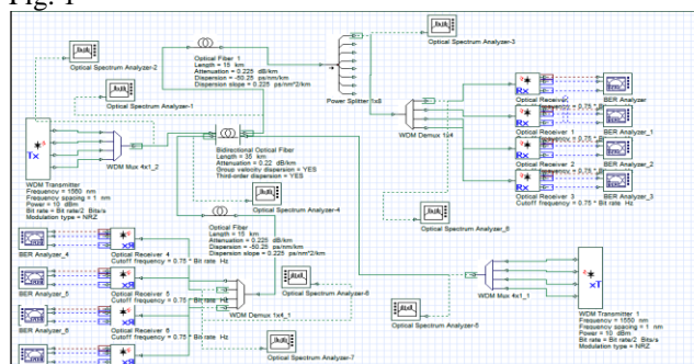
Figure 1: System design with simulation of C-band WDM-PON layout
