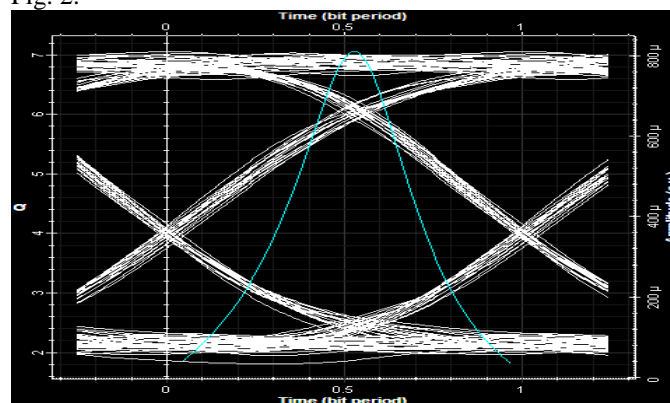
Figure 4: Eye diagram at ONU
