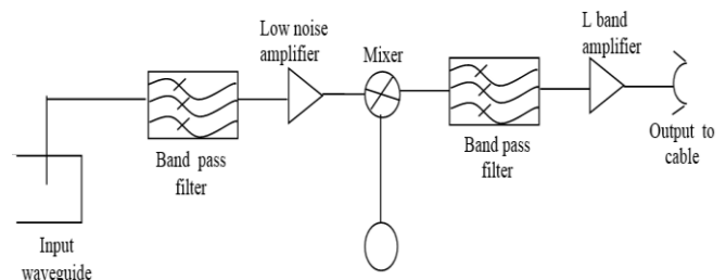
Fig. 1.0: Low noise block down converter diagram
