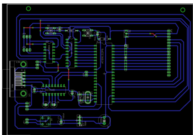
Figure 4: End Device Board Diagram
