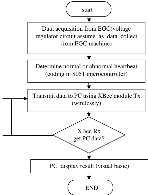
Figure 2: Flow Chart of Project Design
