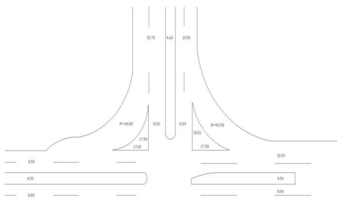
Figure 4.-[Existing T-junction geometry]
