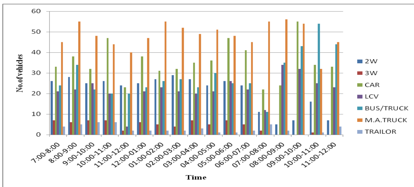
Chart-2. [Shamalaji to By-pass No. of vehicles versus Time graph]
