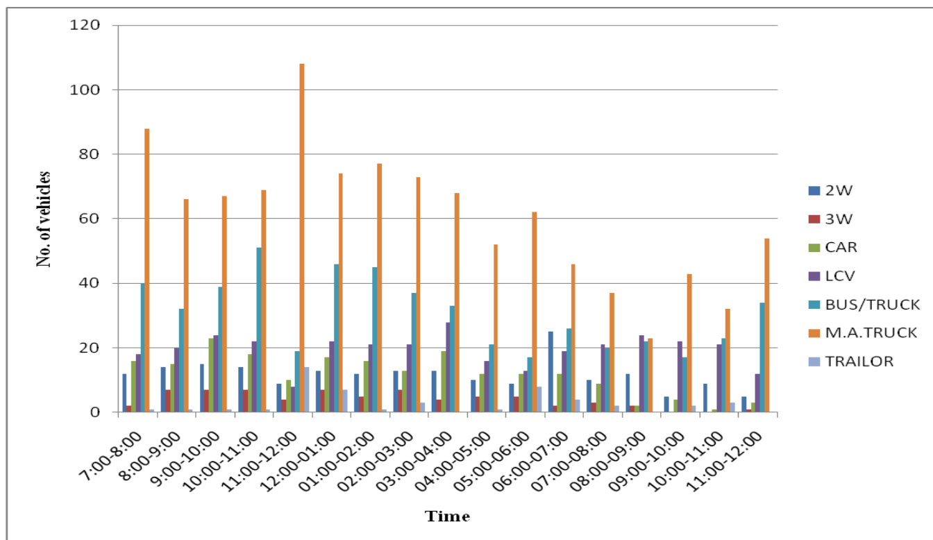
Chart-1. [By-pass to Shamalaji No. of vehicles versus Time graph]
