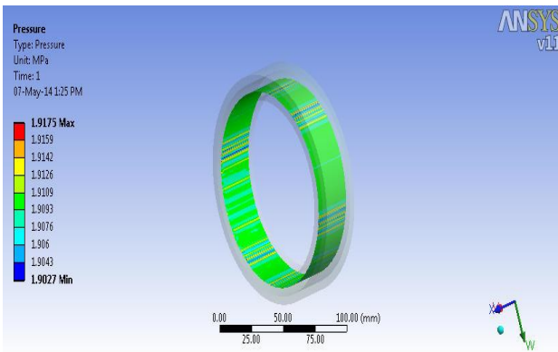
Fig 7. Contact pressure (Ps12)
