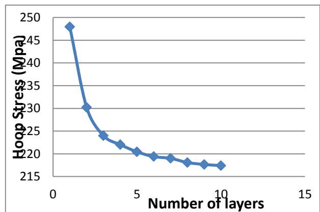
Fig 10.Effect of Number of layers on hoop stress
