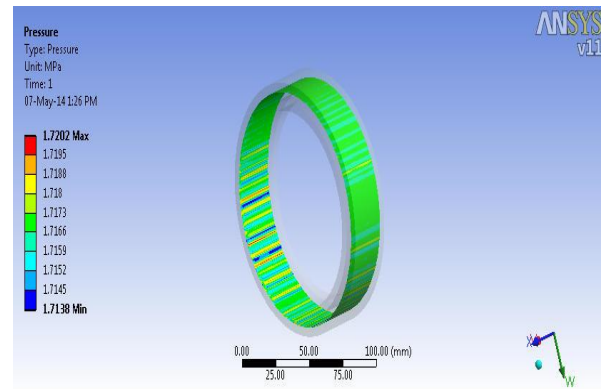
Fig 8. Contact pressure (Ps23)
