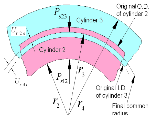
Fig 3. Interference between layer 2 & 3
