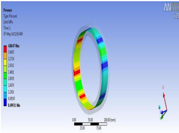
Fig 5. Contact pressure (Ps12)
