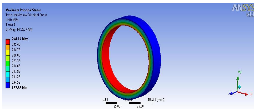
Fig 4. Hoop stresses
