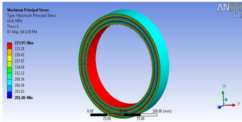
Fig 9. Resultant hoop stresses
