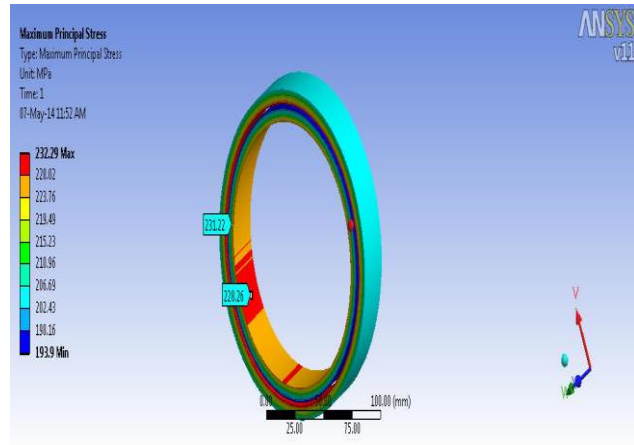
Fig 6. Resultant hoop stresses
