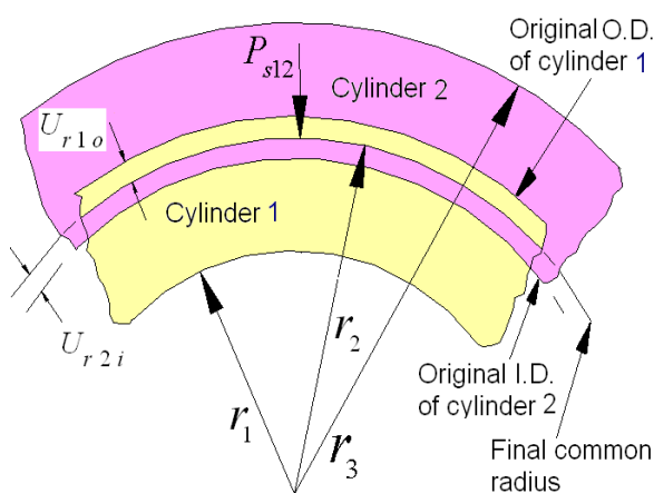
Fig 2. Interference between layer 1 & 2
