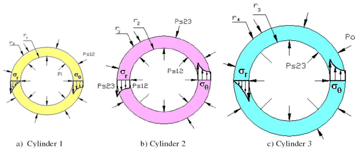
Fig 1. Radial and hoop stress distribution
