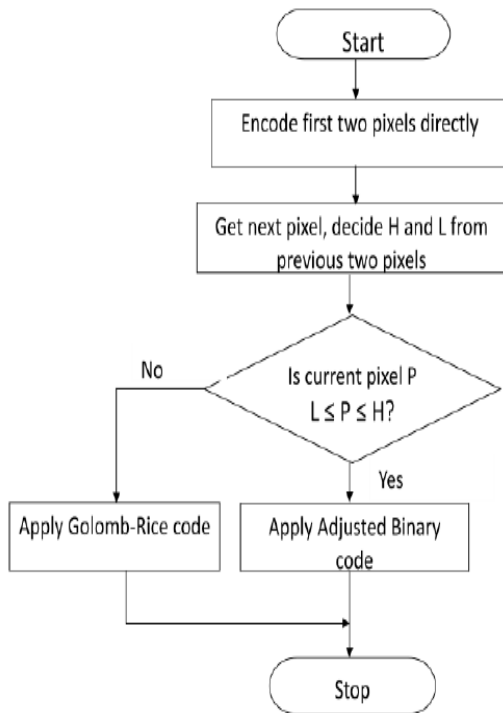
Fig.3 Flowchart for the FELICS Algorithm
