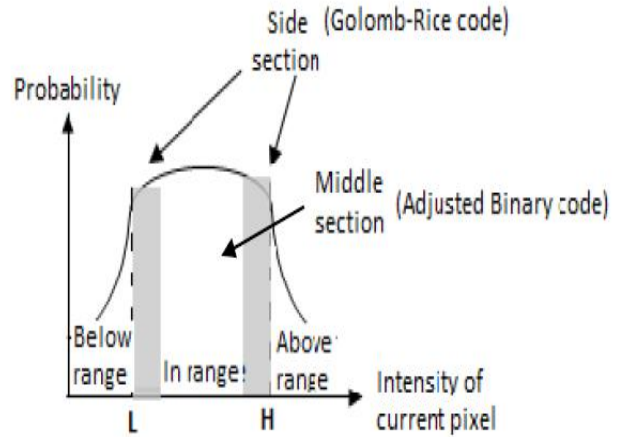
Fig.4 Probability distribution model in FELICS
