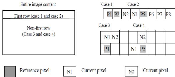
Fig.2 Illustration of prediction template in FELICS
