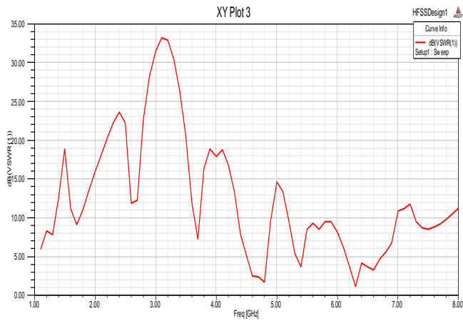
Figure 9: VSWR for first iteration
