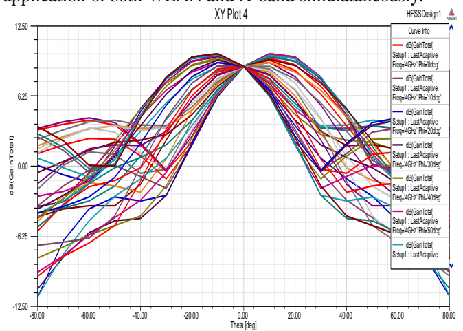
Figure 7: Gain for first iteration
