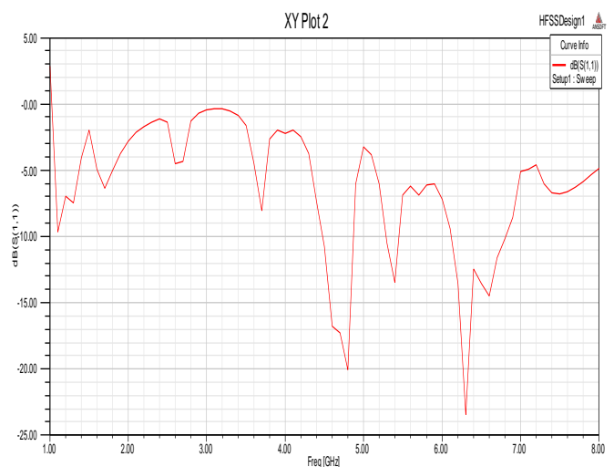
Figure 8: Return loss for first iteration
