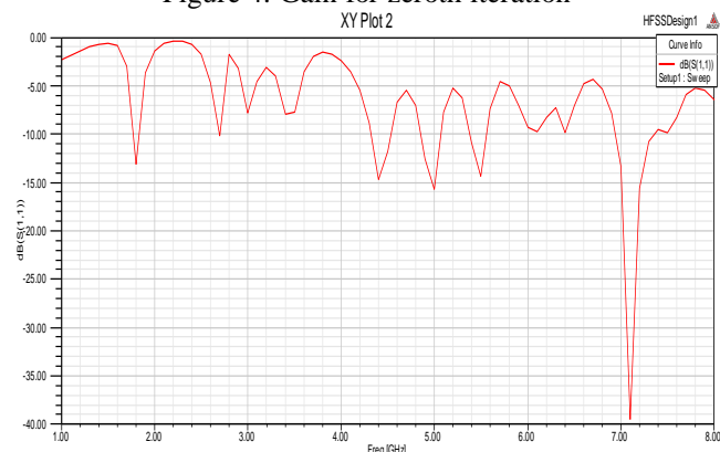
Figure 5: Return loss for zeroth iteration
