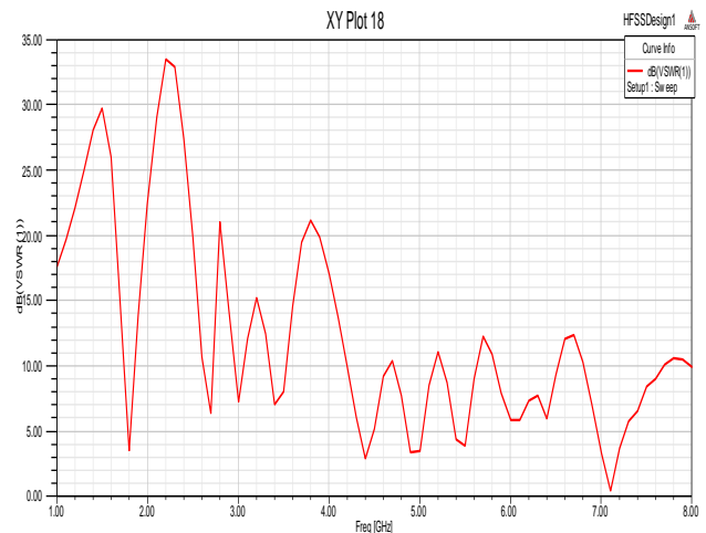
Figure 6: VSWR for zeroth iteration
