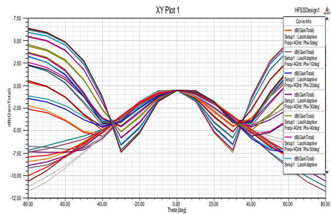
Figure 4: Gain for zeroth iteration
