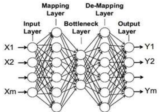
Figure 11. Structure of AANN
