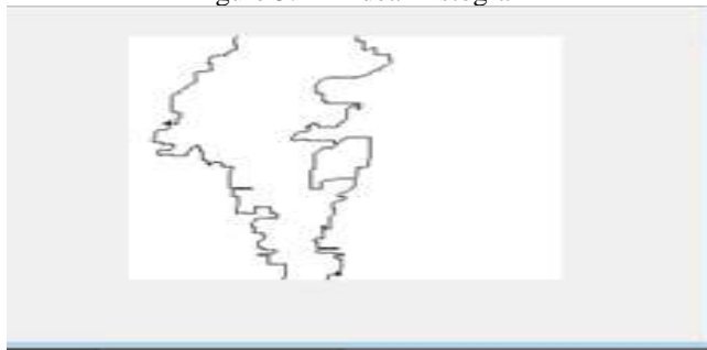
Figure 6. Segmentation
