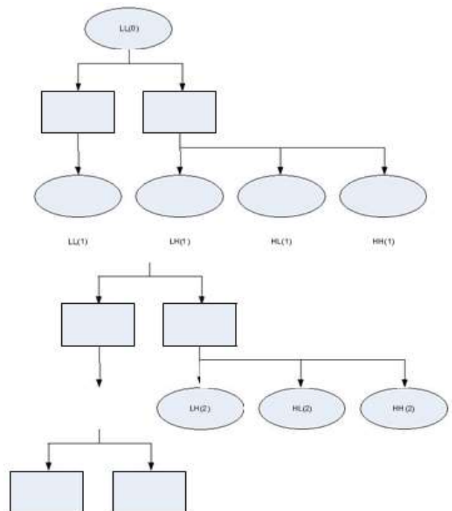
Figure 9. Two level decomposition by two-dimensional wavelet
