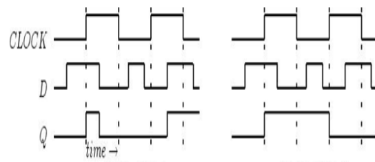
Fig 1 (a) Active High latch (b) Positive Edge Triggered Flip-Flop
