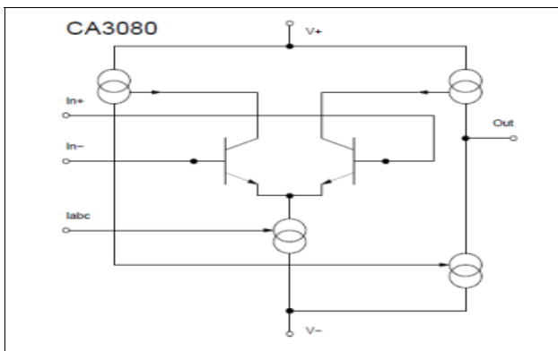
Fig 15: CA3080
