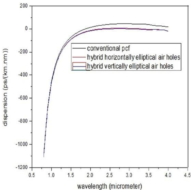
Figure 8. Shows the comparison of chro matic dispersion of the proposed As 2 Se 3 glass PCF and conventional As 2 Se 3 glass PCF when pitch "Λ"= 1.75 μm.
