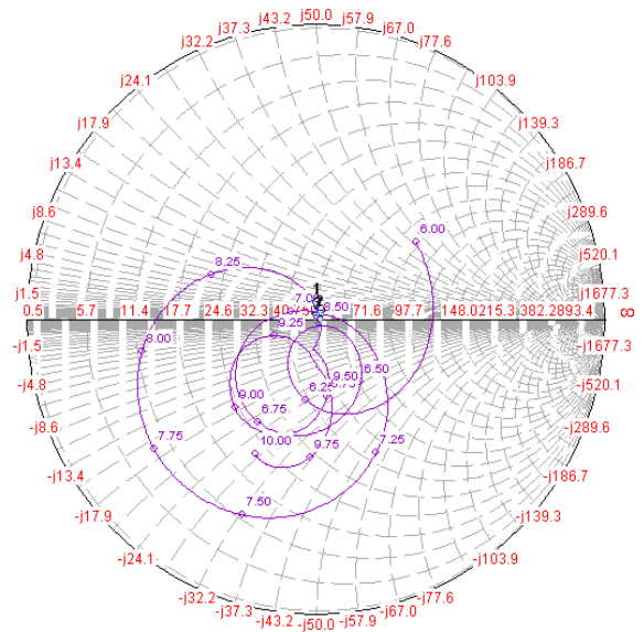
Fig 5: Impedance Matching Measurement
