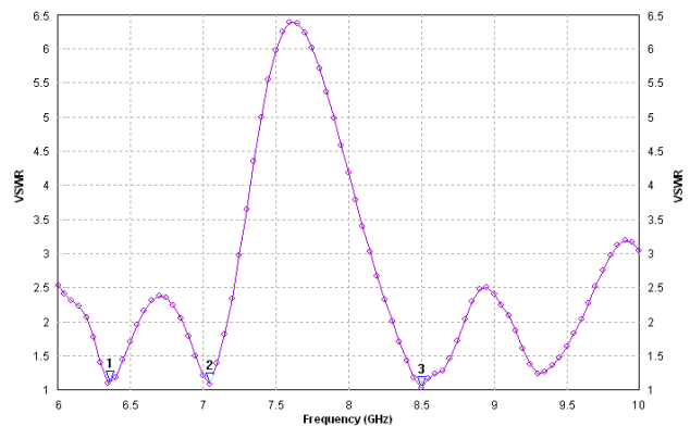
Fig 6:VSWR Measurement
